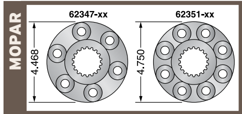
P/N 62347-XX 6-Bolt P/N 62351-XX 8-Bolt, Hemi
